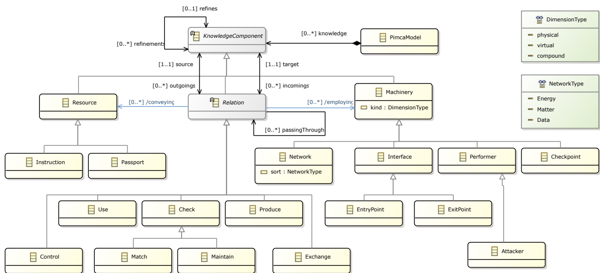
Figure 2: Pimca metamodel.
