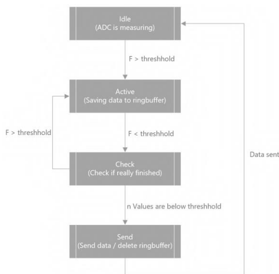
Figure 6: State Machine Measurement.
