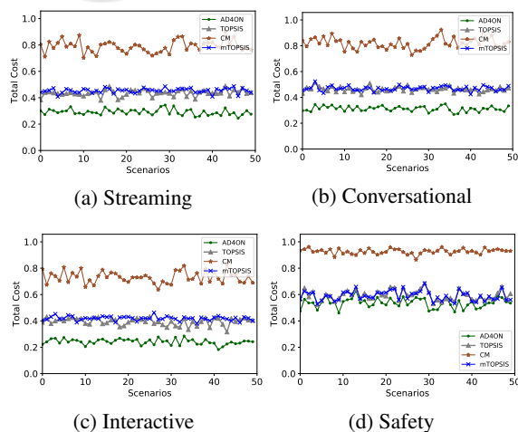
Figure 4: Total Cost.
