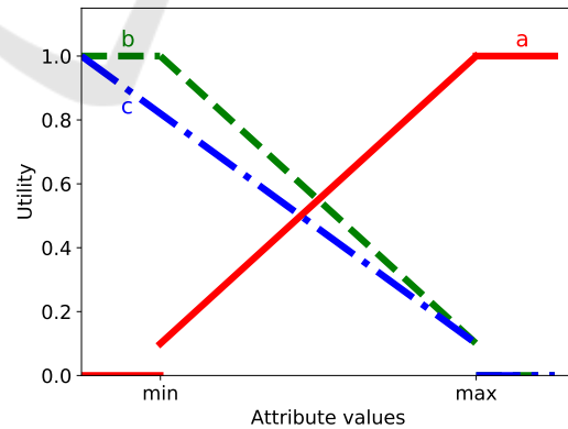
Figure 1: Utility functions.
