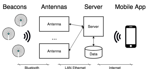
Figure 2: Architecture of the proposed indoor localization system.
