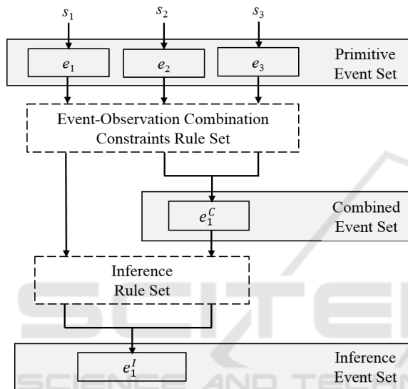
Figure 1: An illustration of the event model M^* using primitive and combined event-observations to infer an inferred event.
