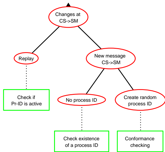
Figure 3: Attacks aiming at creating a shutdown message from the control system (CS) to the smart meter (SM) at the channel between them and the corresponding detection methods.
