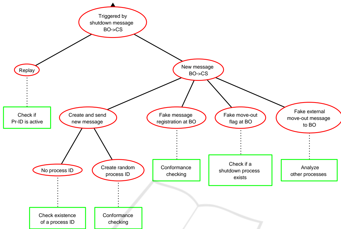
Figure 5: Attacks aiming at creating a shutdown message from the backoffice (BO) to the control system (CS) and the corresponding detection methods.
