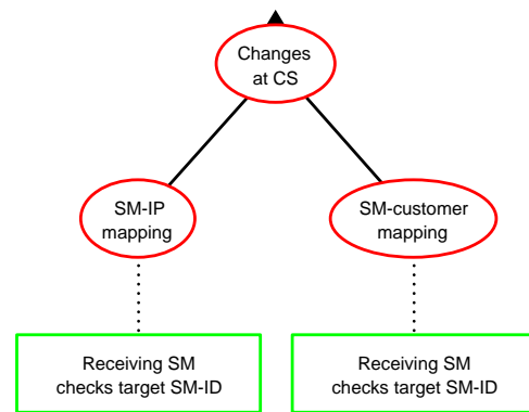
Figure 4: Attacks aiming at creating a shutdown message from the control system (CS) to the smart meter (SM) by changes at the CS and the corresponding detection methods.
