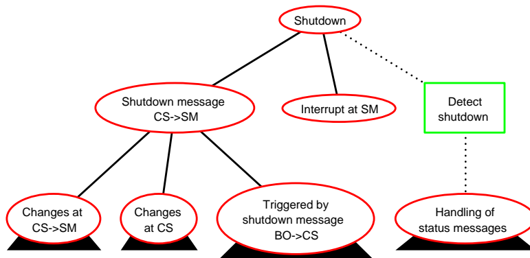
Figure 2: Top levels of the attack-defense tree.
