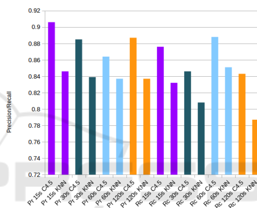
(b) Scenario A NON-VPN Precision and Recall
