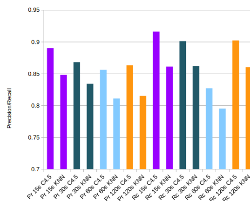
(a) Scenario A VPN Precision and Recall
