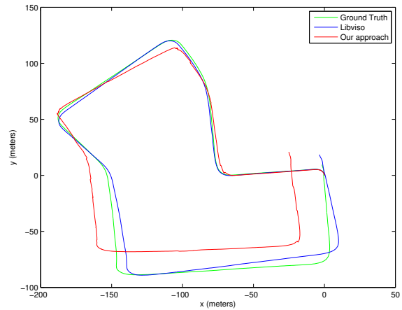
Figure 10: Evolving trajectory of the KITTI sequence. One can observe that our approach (red) performs comparable to Libviso (blue).
