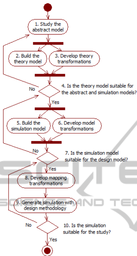
Figure 2: MDE process for traffic simulations.
