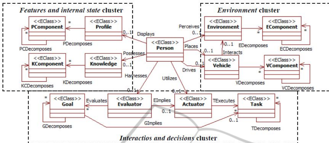
Figure 1: Excerpt of the traffic metamodel. Dotted rectangles indicate the main conceptual clusters. Inverse references are available for all the depicted associations.
