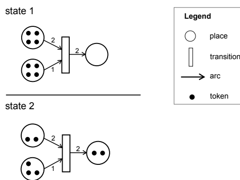
Figure 2: Sample of firing a transition.
