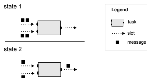
Figure 1: Sample of task execution.
