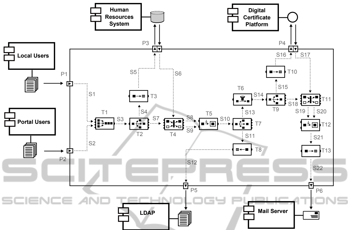
Figure 11: The Huelva's County Council conceptual model for the integration problem.
