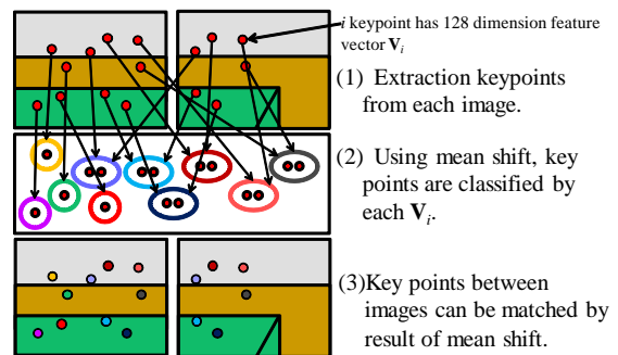
Figure 3: Process of classifying keypoints.
