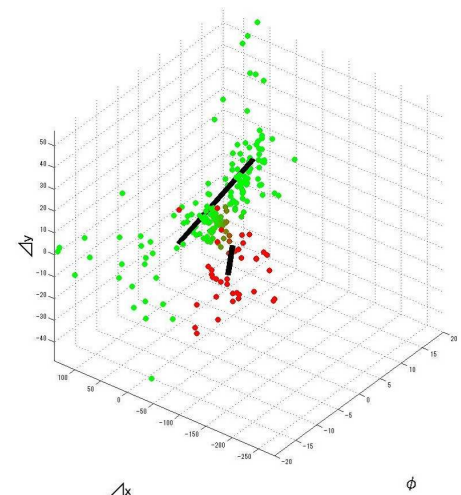
(c) Result of NGnet 3.
