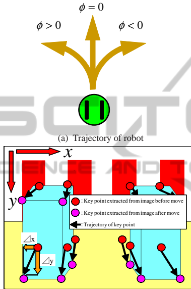
Figure 6: Example of collecting data.
