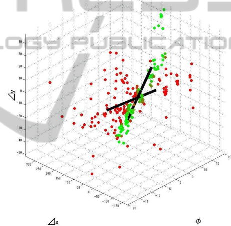
(b) Result of NGnet 2.
