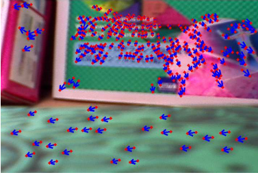
Figure 5: Example of motions of keypoints.
