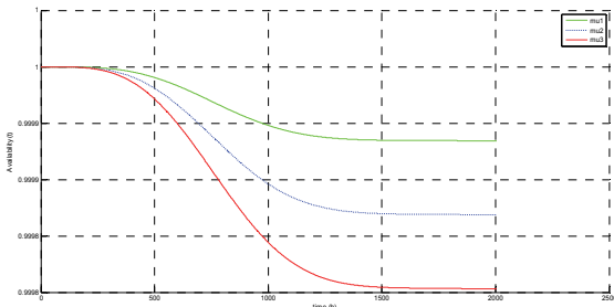
Figure 10: Availability behaviour of the 2003+3 consecutive failures configuration considering 16, 32 and 48h as the inverses of three different repair rates \mu .
