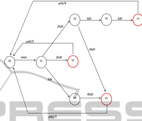
Figure 7: State space representation of the MM of the 3006 + 2 consecutive failures configuration where S2, S5 and S7 represent the failed cases.
