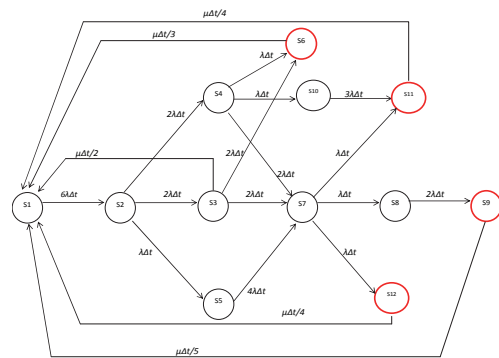
Figure 8: State space representation of the MM of the 2006 + 3 consecutive failures configuration where S6, S9, S11 and S12 represent the failed cases.
