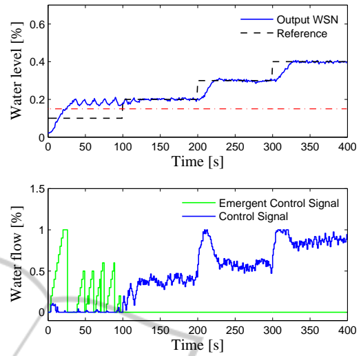
Figure 6: MIMO system working out of limits Tank 2.
