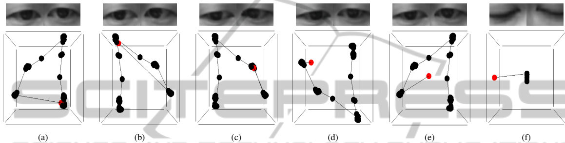
Figure 5: Projection of the training samples plus new eye input of different movements by by Laplacian Eigenmaps ( t=700 ). (Red point represents the new input data, black points represents the training samples).
