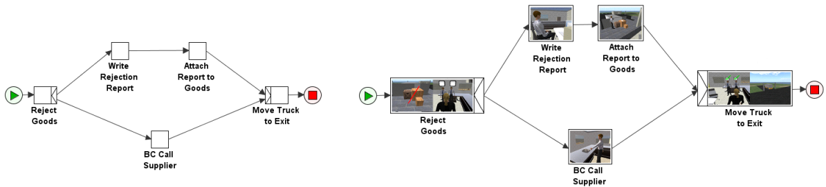
Figure 3: Left: The basic YAWL version of the Goods Rejection model. Right: The annotated model.
