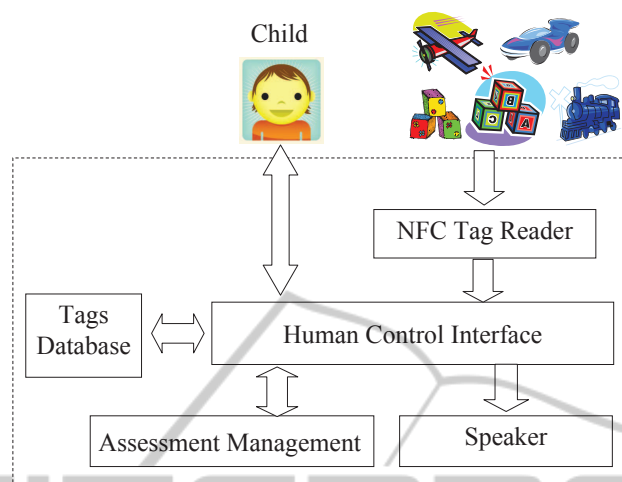
Fig. 3. Application high level architecture.
