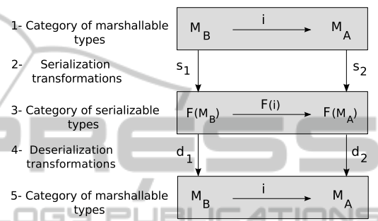
Figure 4: Fundamental Diagram for Serialization and Deserialization.
