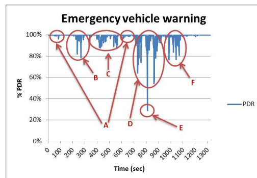
Figure 6: Emergency vehicle warning test results.
