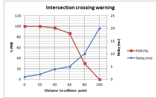
Figure 4: Intersection crossing warning test results.
