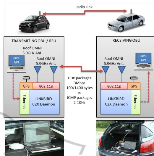
Figure 2: Hardware Setup.
