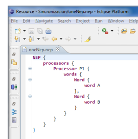
Figure 5: Textual editor window automatically updated by the environment.
