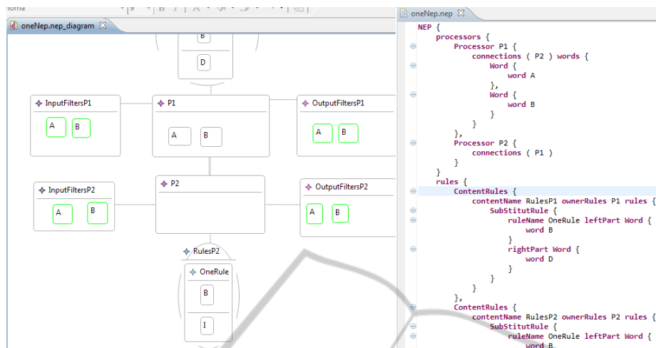
Figure 2: Eclipse windows showing both, the visual and Xtext default textual appearance of the simplest example of NEP.
