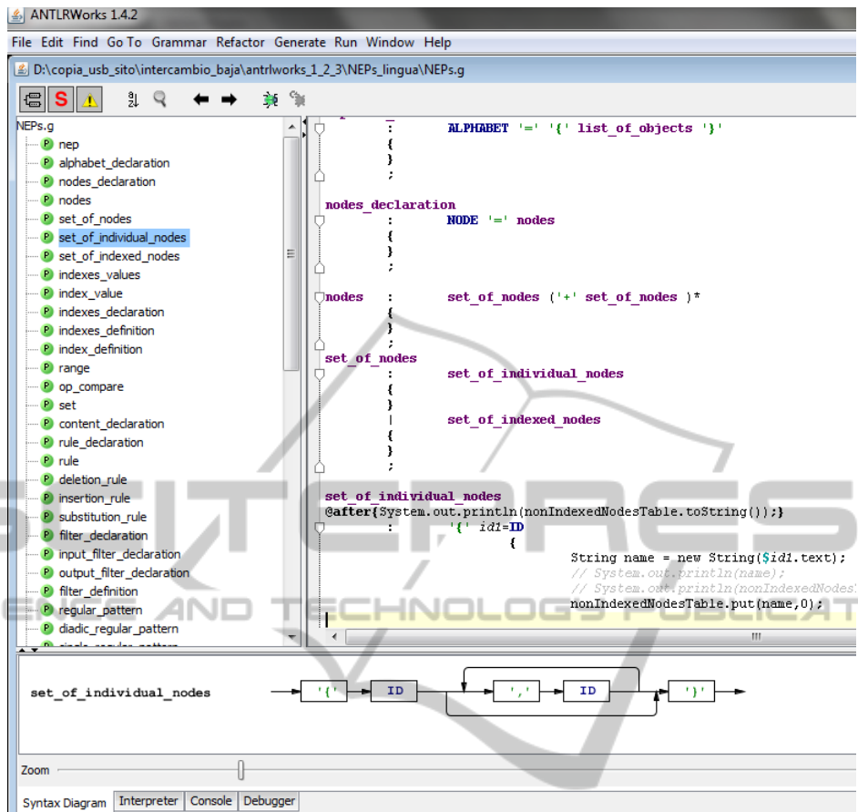
Figure 1: ANTLR window showing some of the elements of the LL(*) grammar for NEPsLingua.
