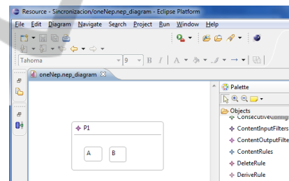
Figure 4: Visual editor window showing a NEP with only one processor: it contains the strings "A" and "B".
