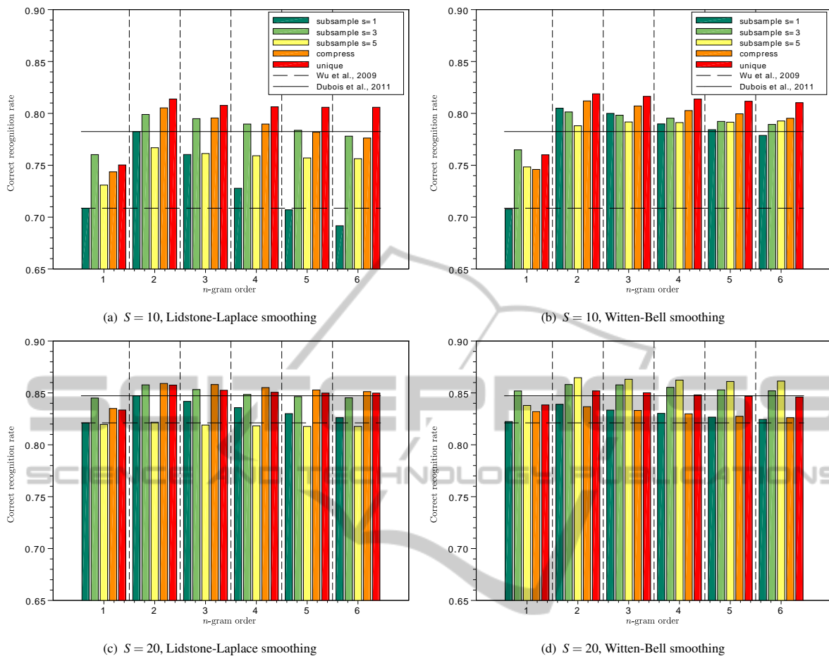
Figure 2: Results on the instance recognition task. The vertical axis is the correct recognition rate (in %). The horizontal axis is the value of n . Upper-row: results for S = 10 . Lower row: results for S = 20 . Left column: results for Lidstone-Laplace smoothing. Right column: results for Witten-Bell smoothing.
