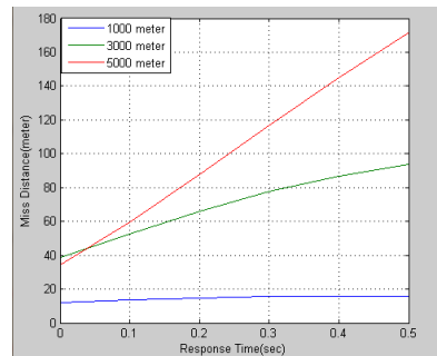
Figure 4: The miss distance as a function of the computer response time for different relative ranges at which the target starts to escape.
