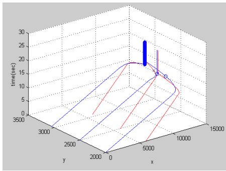
Figure 6: Simulation results for OCAA with a computer response time of 0.01s. Around 17s to 18s all three missile-target pairs stop moving, i.e., all three missiles entered their explosion range and hit their targets.
