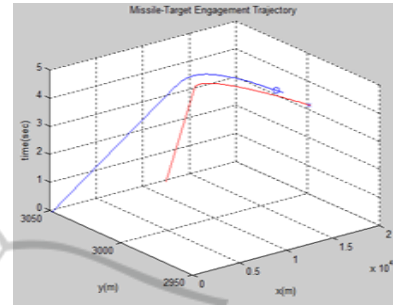
Figure 2: The trajectories of the missile and the target for a computer response time of 0.01s.
