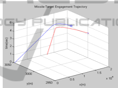
Figure 3: The trajectories of the missile and the target for a computer response time of 0.1s.
