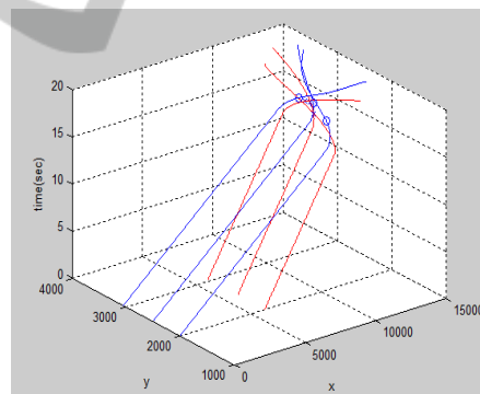
Figure 5: Simulation results for PNG, with a computer response of 0.01s. Blue (Red) lines are missile (target) trajectories. Once the missile enters its explosion range, it explodes, and this missile and its target stop moving.
