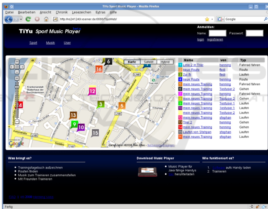
Figure 3: TIYU website.
