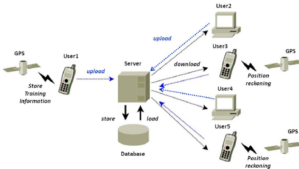
Figure 2: Architecture of the TIYU system.
