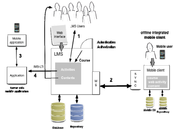
Figure 1: Architecture to integrate LMS with external mobile applications.
