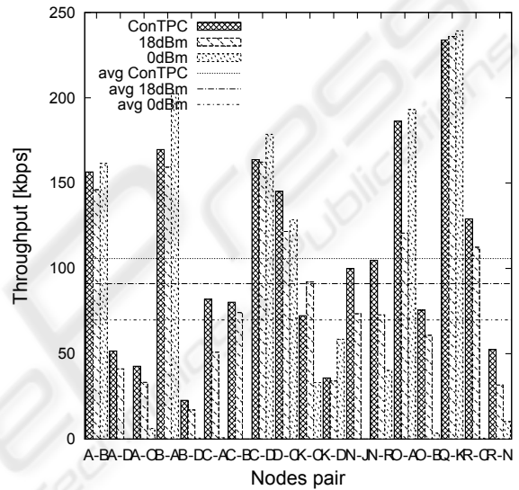
Figure 12: Throughput observed on 11 node testbed.
