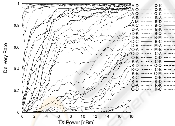
Figure 5: Delivery rate vs TX power.
