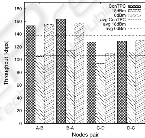
Figure 9: Throughput observed in disjoint case.
