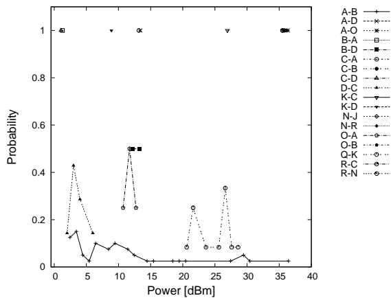
Figure 13: Power level selection PDF for links of 11 node testbed.
