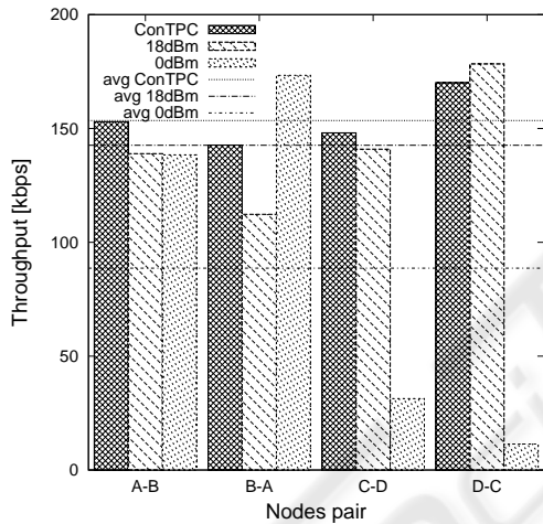
Figure 11: Throughput observed in 4 nodes case.
