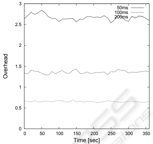
Figure 14: ConTPC overhead.
