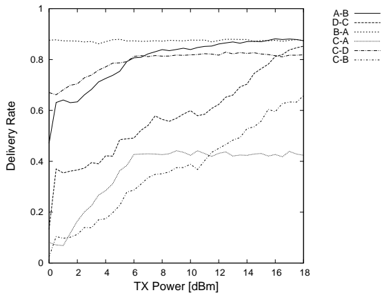
Figure 10: Delivery rate characteristics observed in 4 nodes case.
