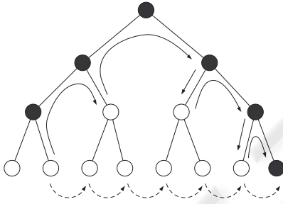
Figure 3: Scanning along the depth subdivision tree. Cells represented by black nodes may intersect with the surface. Cells represented by white nodes do not. The solid arrows show progression by depth-first order. The dotted arrows show progression by breadth-first order.
