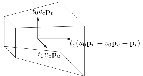
Figure 1: The geometry of a cell. The vectors show the three medial axes of the cell.
