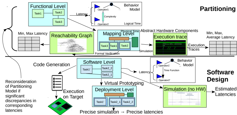
Figure 1: Latency Measurement through the Embedded System Design Process.
