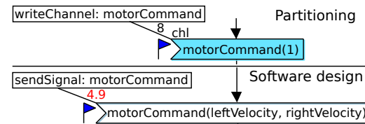
Figure 8: Backtracing latencies.
