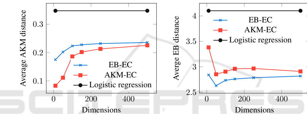
Figure 7: Average AKM and EB distances of embedding classifiers on the test dataset for misclassified samples.
