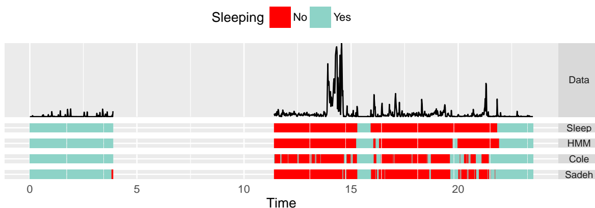
Figure 4: Example classification of one recording period for healthy subjects. Data: Raw acceleration values (lowpass-filtered for depiction). Sleep: Sleep annotations. HMM, Cole, Sadeh: Classification obtained by respective algorithms. In this example, the HMM shows a good classification, while Cole’ and Sadeh’s algorithm overestimate the state sleeping and the number of state transitions.
