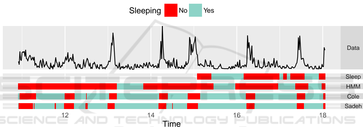
Figure 5: Example classification of one recording period of subjects with dementia. Data: Raw acceleration values (lowpass-filtered for depiction). Sleep: Sleep annotations. HMM, Cole, Sadeh: Classification obtained by respective algorithms. In this example, the HMM shows a balanced sleep/wake classification, while Cole and Sadeh overestimate the state sleeping .
