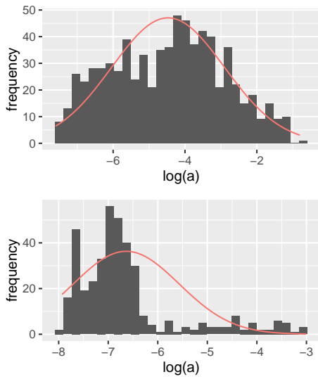
Figure 3: Histogram of sensor data, one recording, class awake (top) and class sleeping (bottom), logarithmic scale. Red line: Empirical log-normal distribution.
