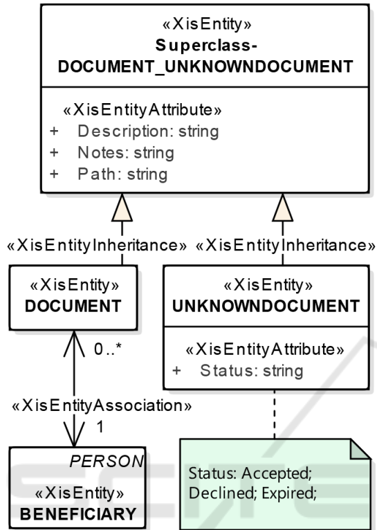
Figure 9: Case Study SS-App XIS* Domain view.
