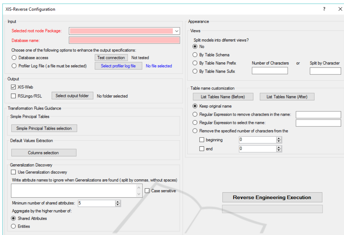
Figure 8: Configuration panel of the tool.
