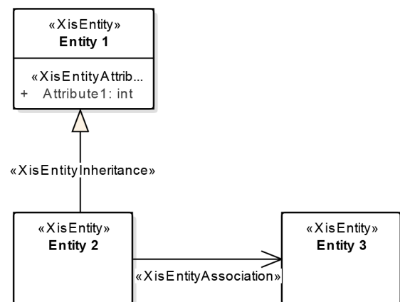
Figure 3: XIS* Domain view.
