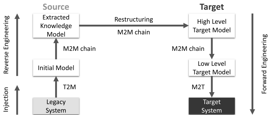
Figure 1: Model-driven reengineering process.
