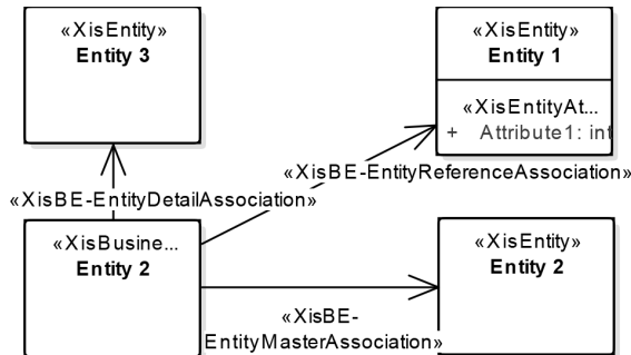
Figure 4: XIS* BusinessEntities view.
