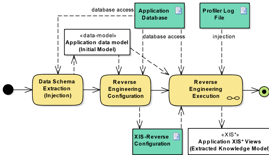
Figure 6: Overview of the XIS-Reverse approach.
