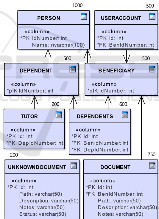
Figure 7: Case Study SS-App data model.
