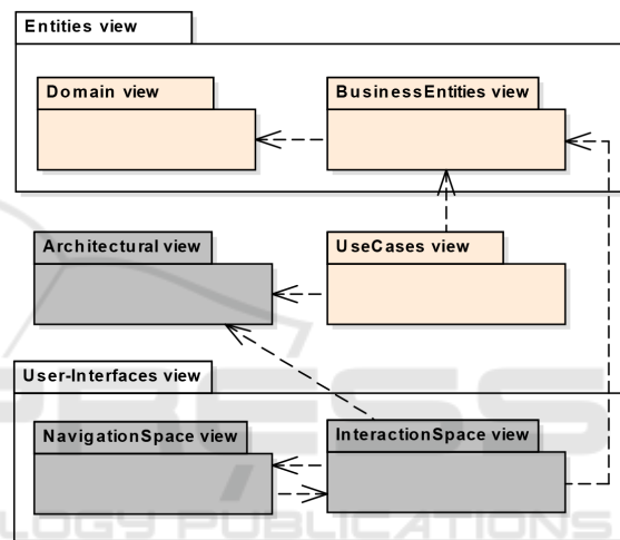
Figure 2: The multi-view organization of XIS*.
