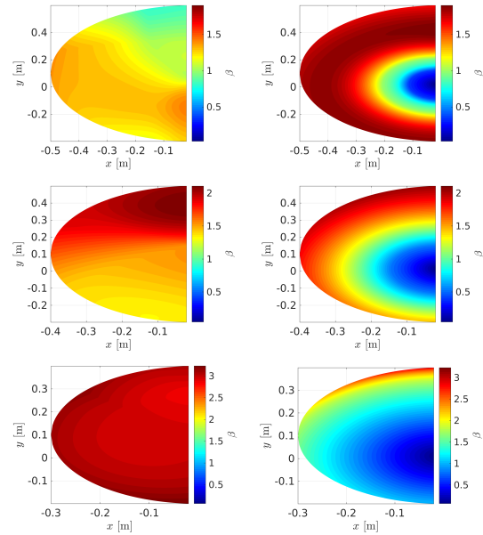
Figure 10: The evolution of the slippage avoidance index in xy -plane when the robot is set in different configurations within the defined workspace I, II and III, presented at the first, second and third row, respectively; while the two kinematics arrangement RPP and YPP are shown on the left and right sides.
