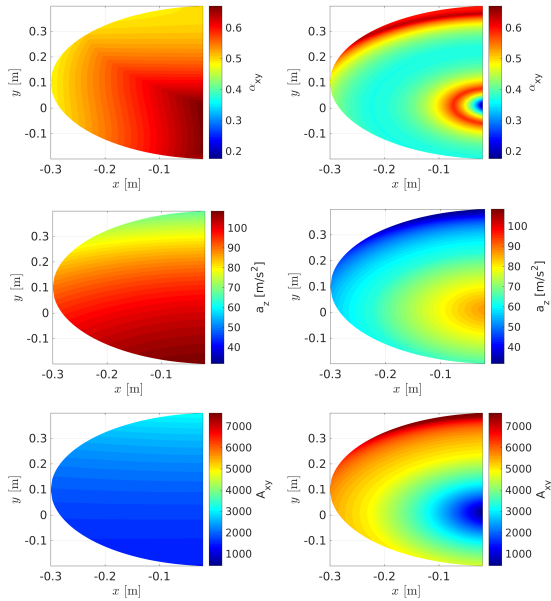
Figure 9: The evolution of the DMP indexes in xy -plane when the robot is set in different configurations within the defined workspace III, for two kinematics arrangement: The RPP torques on the left side, and the YPP torques on the right side.
