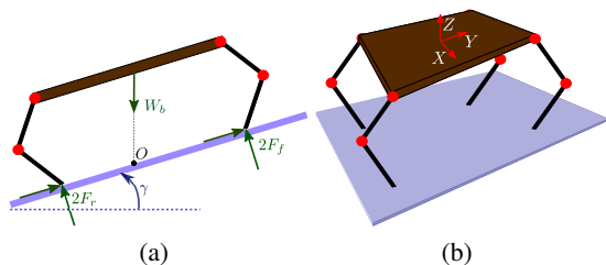
Figure 2: Schematics of the quadrupedal robot to be discussed in this work, without demonstrating the first joint of the leg (hip yaw/roll).
