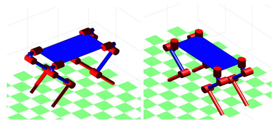
(a) Roll-Pitch-Pitch leg (b) Yaw-Pitch-Pitch leg
