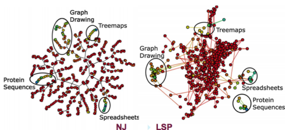
Figure 6: Comparison of INFOVIS04 document data set map using Neighbor Joining and LSP projections: Four different topics of information visualization are identified by coloring points. Figure is taken from (Cuadros et al., 2007).
