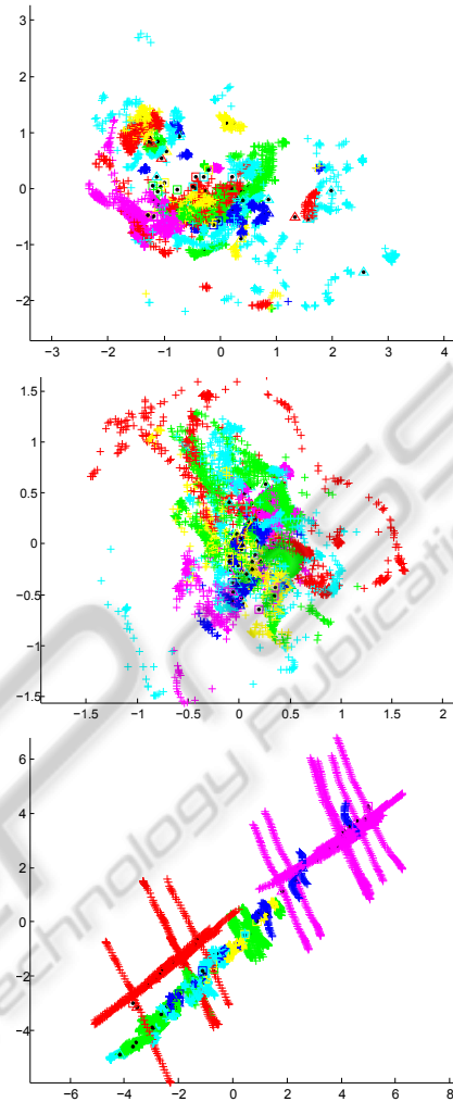
Figure 3: Top Latent-space representation considering Euler Angles representation and PPCA initialization, Middle Latent-space representation considering Unit-Quaternion representation and PPCA initialization, Bottom Latent-space representation considering 3D Point Cloud representation and PPCA initialization.
