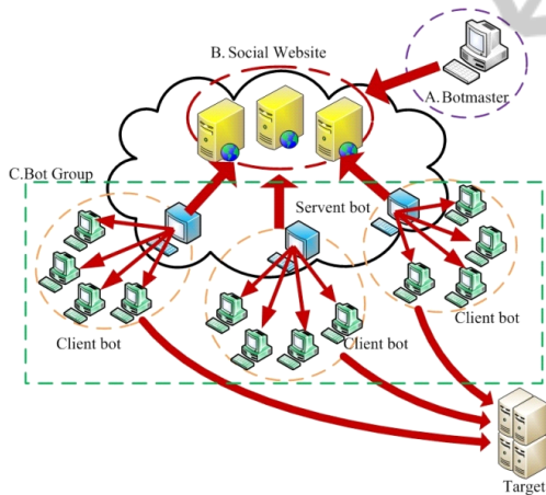
Figure 1: The proposed hybrid P2P botnet 2.0 structure.
