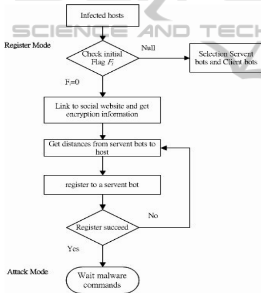
Figure 3: Steps of client bots process: register mode and attack mode.
