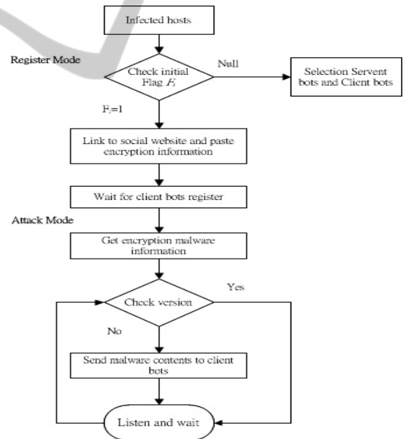
Figure 2: Steps of servent bots process: register mode and attack mode.
