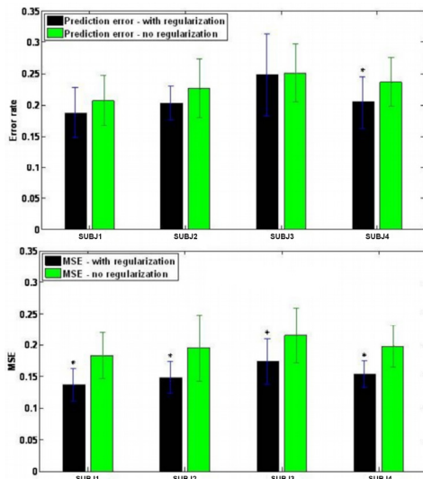
Figure 9: Prediction error (Error rate and MSE) received for 3 best time points chosen, with and without regularization. These figures show that results with regularization are significantly better ( *p < 0.05 ).
