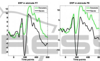
Figure 6: ERP in electrodes P7 and P8.
