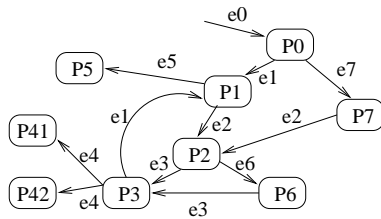
Figure 4: Testing order.
