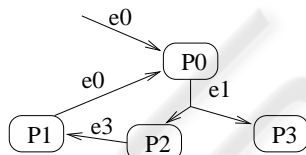
Figure 2: Plan Dependencies.
