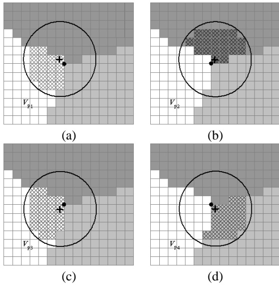
Figure 3: FLAM area associated to four pixels around a junction point and the computed variations. (a) Variation at pixel p_1 , \mathcal{V}_{p_1} (b) Variation at pixel p_2 , \mathcal{V}_{p_2} (c) Variation at pixel p_3 , \mathcal{V}_{p_3} (d) Variation at pixel p_4 , \mathcal{V}_{p_4} .
