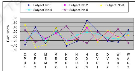
Figure 3: Part-worth \lambda_{ki} of five subjects estimated with proposed Method 2.
