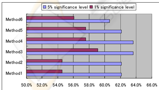
Figure 4: Percentage of subjects for whom correlation between preferences estimated with conjoint analysis and proposed methods was significant at 1% and 5% levels.
