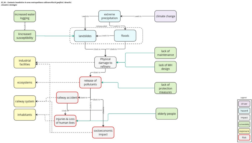
Figure 11: Storyline 4.
