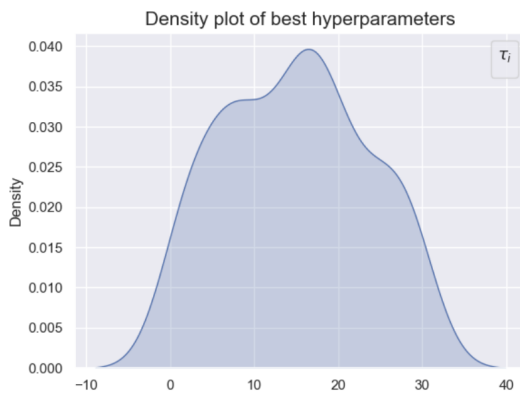
Figure 3: Density plot of \tau values across different lineups, showing the distribution and variation in optimized decay rates.
