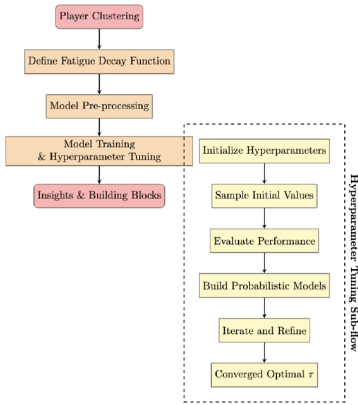
Figure 2: Flowchart for Lineup Optimization Process with Hyperparameter Tuning Sub-flow, optimizing the \tau values to incorporate within the decay function.
