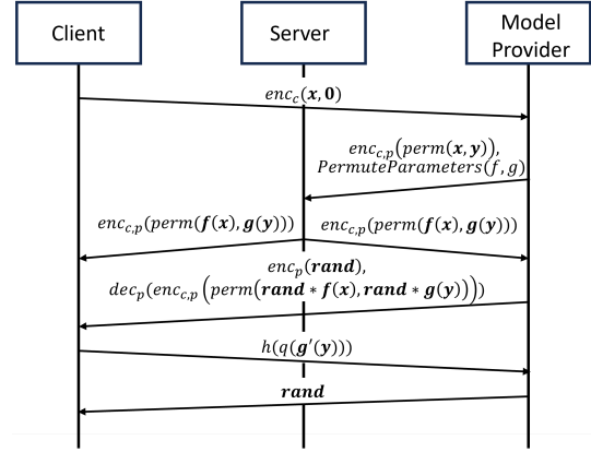
Figure 2: SONNI sequence diagram.
