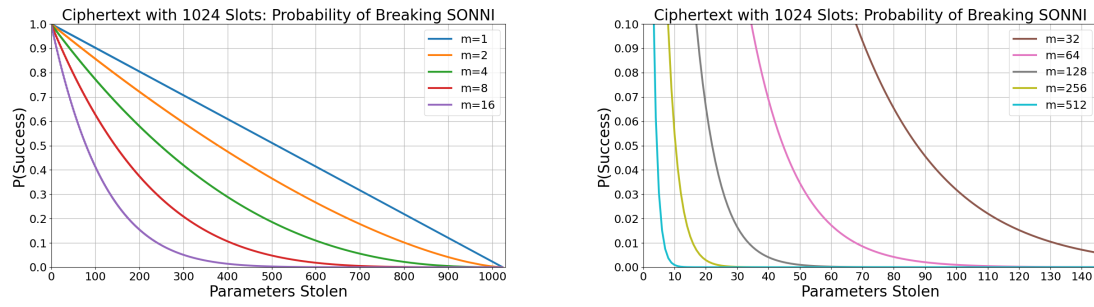
Figure 3: Probability of performing a Silver Platter attack without being detected based on the number of ciphertext slots dedicated to checked values.
