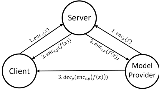
Figure 1: Standard Outsourced Oblivious Neural Network Inference Model.
