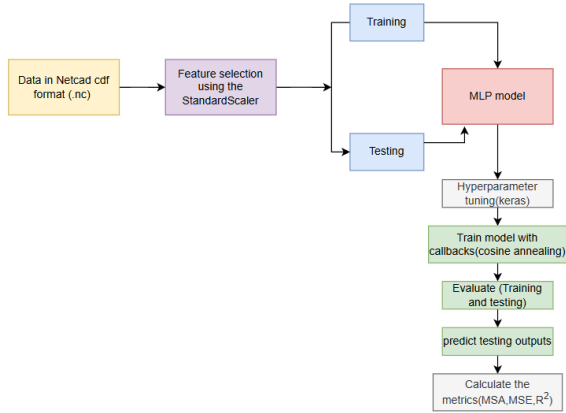
Figure 2: Workflow of the weather prediction model using MLP.
