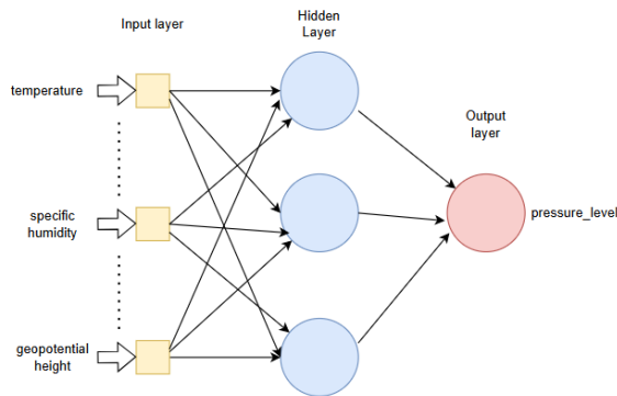
Figure 1: Systematic diagram of MLP: Depicting the interconnected layers responsible for feature selection and prediction.
