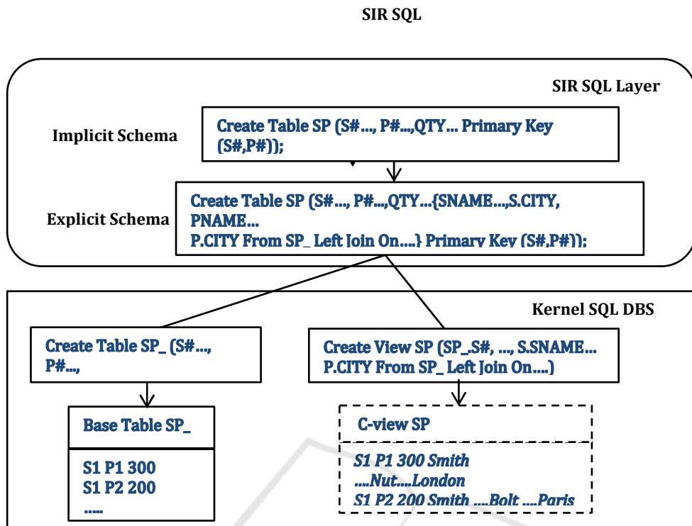
Figure 4. Canonical Implementation of S_P1.SP base table with the actual content within kernel SQL DBS. As for any SQL view, C-view SP content is basically virtual.
