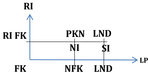
Figure 3 SIR SQL Foreign Keys. RI FK enforces RI. PKN FKs imply NI, NFKs in particular. LND FKs specify SI. An FK can be RI FK only or LP FK only, or both.
