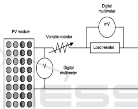
Figure 5: Schematic of PV module measurement system.
