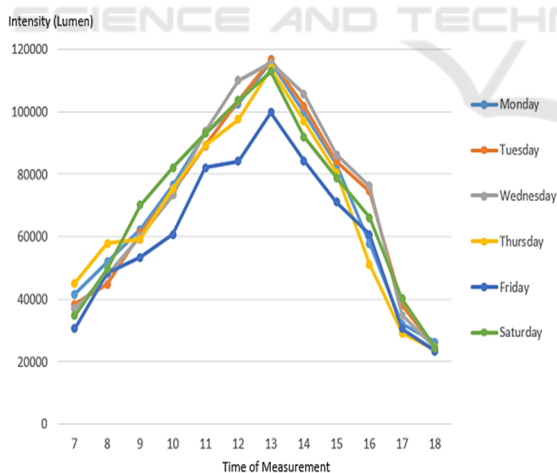
Figure 7: Curve of polar panel intensity average.
