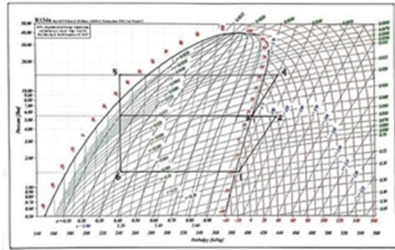
Figure 5: P-h Diagram system with intercooler.
