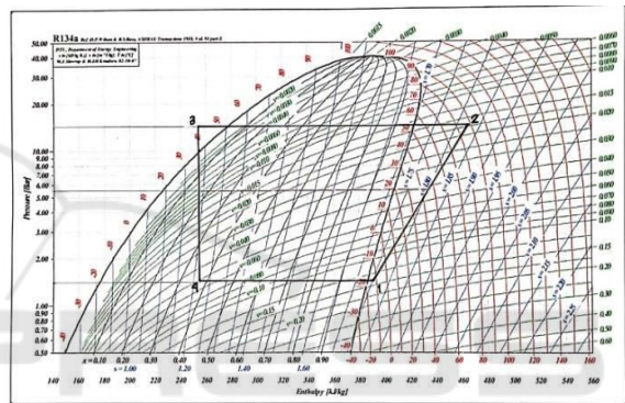
Figure 6: P-h Diagram system without intercooler
