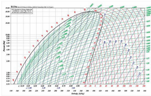
Figure 3: A P - h Diagram.
