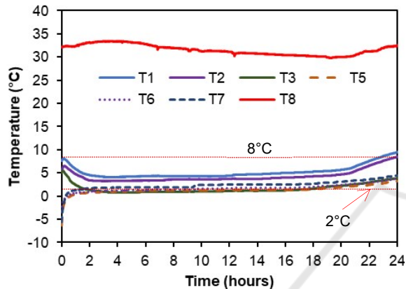
Figure 6: Vaccine box test results using bio-Nano PCM with total mass of 2.7 kg.
