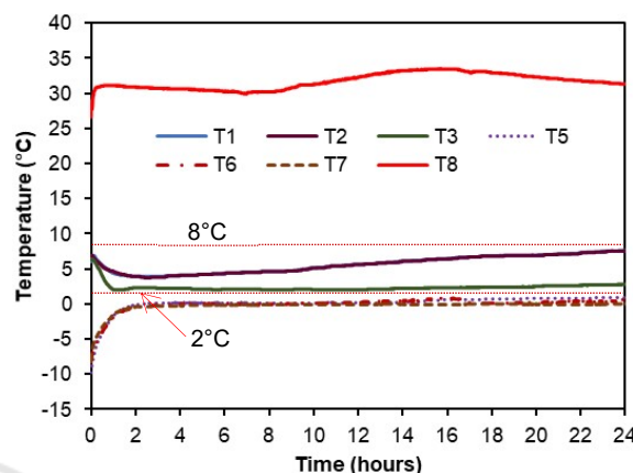
Figure 5: Vaccine carrier test results utilizing bio-Nano PCM with total mass of 3.2 kg.
