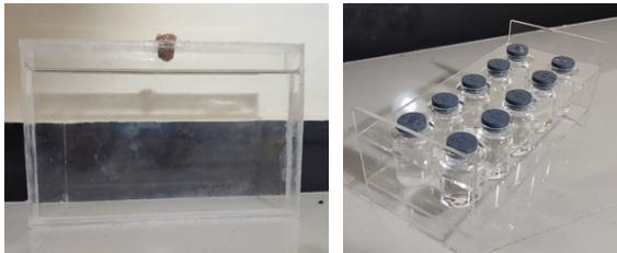
Figure 2: The bio-Nano PCM containers and vaccine bottle holder.
