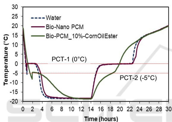
Figure 4: Charging and discharging test results of PCM alternatives.
