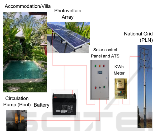
Figure 1: Design of hybrid energy system photovoltaic and national grid (PLN).
