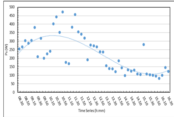
Figure 5: Variation of daily power output of photovoltaic.
