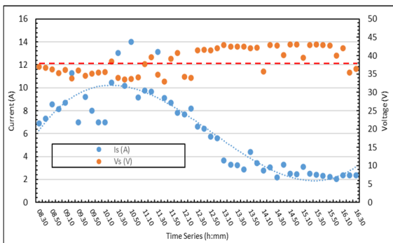
Figure 4: Variation of daily Current (I) and Voltage (V) of the photovoltaic array.
