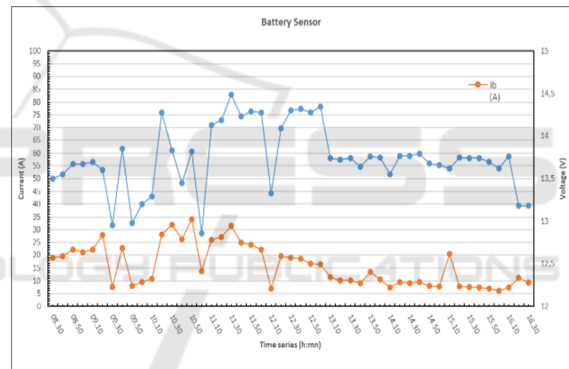
Figure 6: Batterie sensor of Voltage (V) and Current (I).
