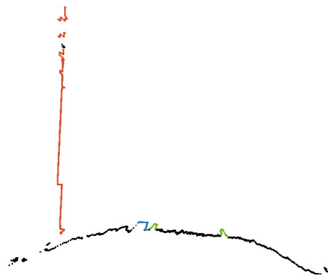
Figure 8: Exemplary semantic classification results of the scan line shown in Figure 6b using U-Net. Points are colored based on semantic class: Signal (red), rail (green), axle counter (blue), other (black).
