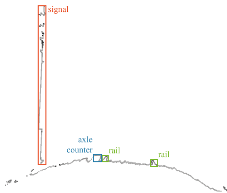
Figure 7: Exemplary semantic classification results of the scan line shown in Figure 6b using YOLO. Bounding boxes are placed around identified objects.
