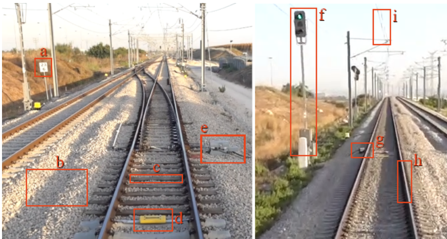
Figure 3: Typical objects found in railroad environments: Sign (a), ballast (b), tie (c), balise (d), switch motor (e), signal pole (f), axle counter (g), rail (h), catenary (i).
