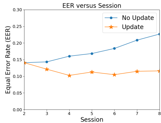
Figure 2: EER versus session averaged across user using the scaled Manhattan distance (Killourhy and Maxion, 2009). When no update strategy is used, the EER is increasing steadily as the testing keystrokes get farther away from the profile. When the profile is updated after each session, the EER does not increase.
