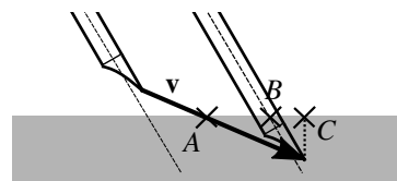
Figure 7: Collision point detection using a ray-casting following the velocity \mathbf{v} . A is our detection point, B is the detection point along the shaft, C is the detection point with minimal distance to the surface of the virtual object.
