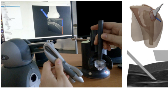
Figure 12: Our simulator which couples a graphical rendering with two haptic devices simulating probe and needle. (up) 3D models (shoulder-probe-needle); (down) zoom on tissue deformation with ultrasound view.
