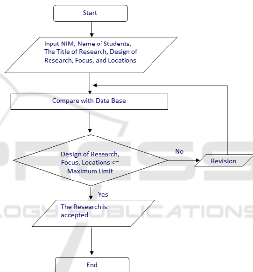
Figure 2: Flow Chart of Thesis Detector.
